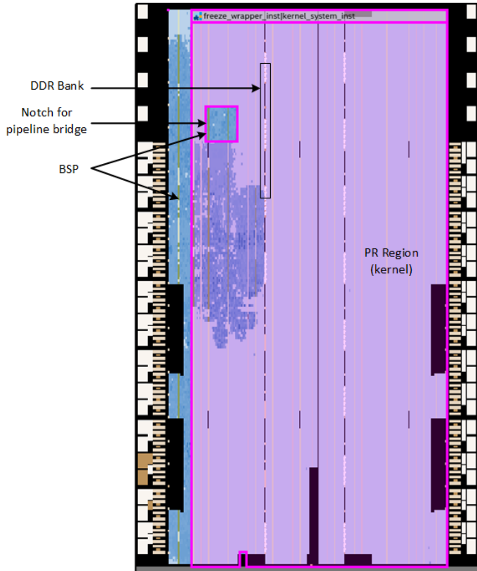
Figure 1. OpenCL BSP Floorplan for Intel Arria® 10 GX in the 17.0 Release
